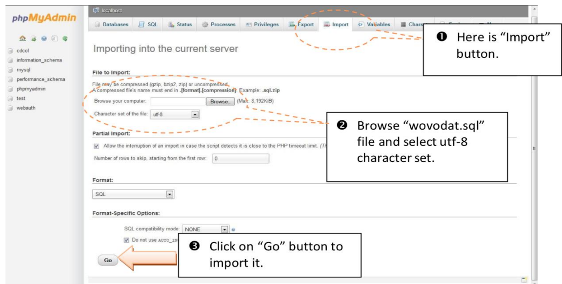
Figure 4. Importing a database into the current server using phpMyAdmin GUI
