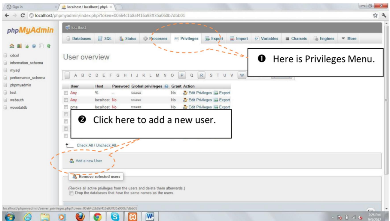
Figure 5. Create new account using phpMyAdmin GUI
